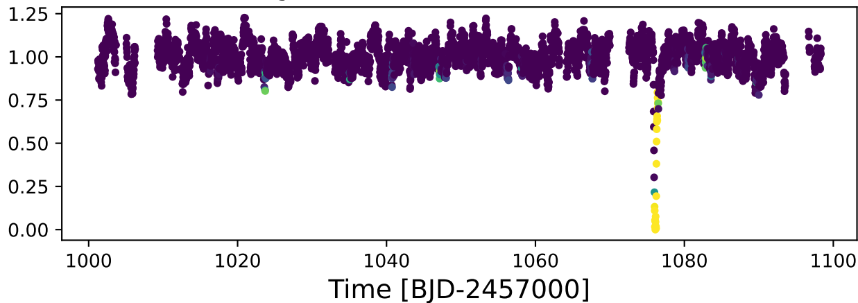
Single Model Predictions - KIC 8072456
