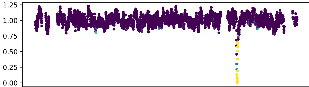
Single Model Predictions - KIC 8072456
